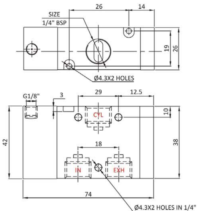
Size : 1/4" BSP (Dimensions are in mm)
